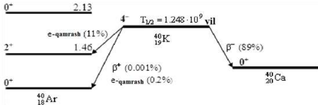
2-rasm. ^{40}\text{K} -izotopining parchalanish sxemasi.
